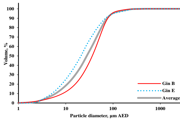
Figure 6. Gin average particle size distributions for the PM captured in the EPA-Method 17 sampler nozzle wash from the mote trash systems.
