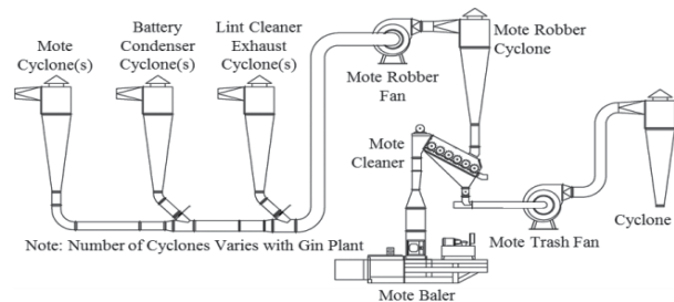
Figure 2. Typical cotton gin mote trash system layout (Courtesy Lummus Corporation, Savannah, GA).
