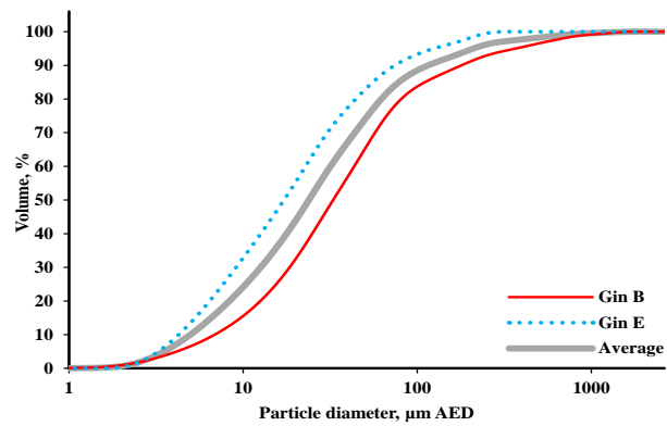
Figure 7. Gin average particle size distributions for the EPA-Method 17 combined filter and wash samples from the mote trash systems.
