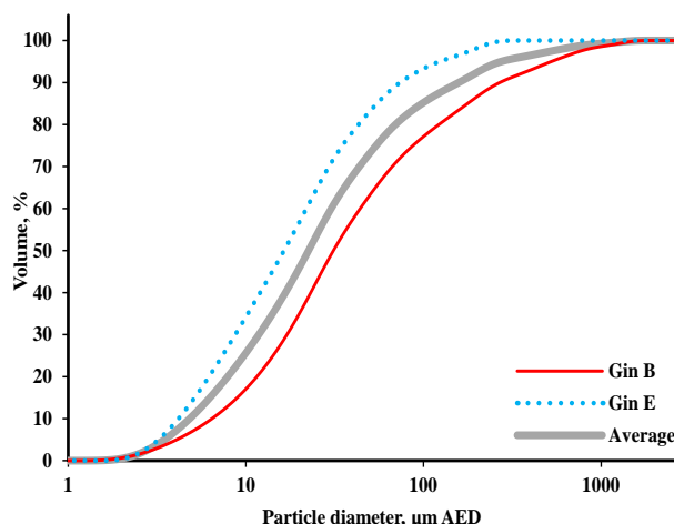
Figure 5. Gin average particle size distributions for the PM captured on a EPA-Method 17 filter from the mote trash systems.
