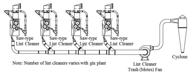
Figure 2. Typical cotton gin combined mote system layout (Courtesy Lummus Corporation, Savannah, GA).
