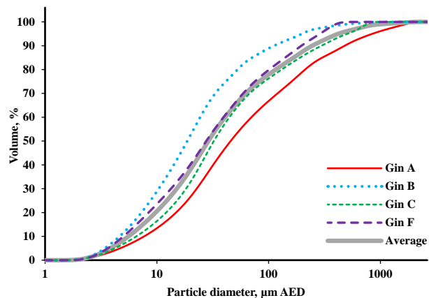
Figure 5. Gin average cumulative particle size distributions for the PM captured on a EPA-Method 17 filter from the 1 st stage lint cleaning systems.
