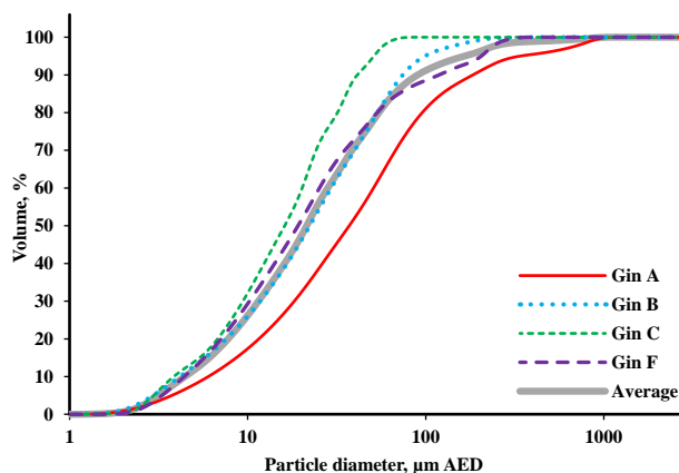
Figure 6. Gin average cumulative particle size distributions for the PM captured in the EPA-Method 17 sampler nozzle wash from the 1 st stage lint cleaning systems.
