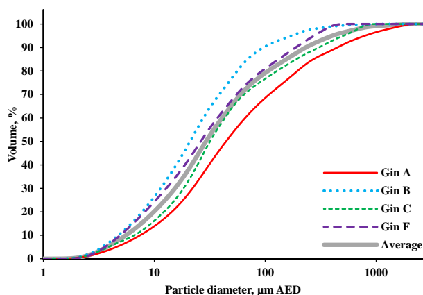
Figure 7. Gin average cumulative particle size distributions for the EPA-Method 17 combined filter and wash samples from the 1 st stage lint cleaning systems.
