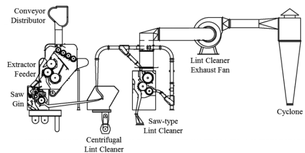
Figure 2. Typical cotton gin 1 st stage lint cleaning system layout (Courtesy Lummus Corporation, Savannah, GA).
