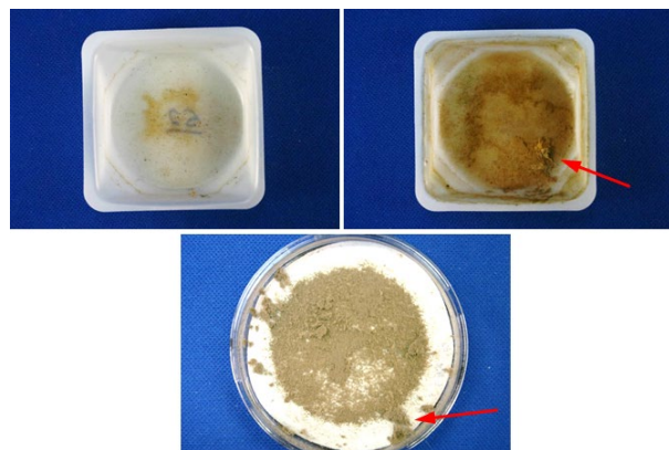
Figure 18. EPA Method 201A filter and sampler head acetone washes from the 2 nd stage seed-cotton cleaning system with lint fibers in the \leq 10 \mu\text{m} wash and on the filter (indicated by arrows). Clockwise from top left: > 10 \mu\text{m} wash, \leq 10 \mu\text{m} wash, and filter.
