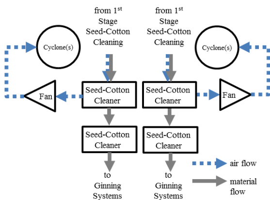
Figure 13. Schematic of split stream, double cleaner 2 nd stage seed-cotton cleaning system without dryer (gin F).
