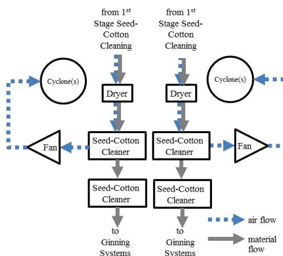
Figure 11. Schematic of split stream, double cleaner 2 nd stage seed-cotton cleaning system with dryer (gin D).
