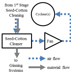
Figure 14. Schematic of single stream, single cleaner 2 nd stage seed-cotton cleaning system without dryer (gin G).
