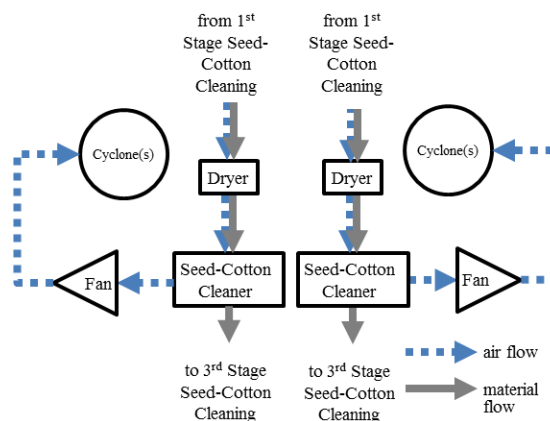
Figure 10. Schematic of split stream, single cleaner 2 nd stage seed-cotton cleaning system with dryer (gin A).
