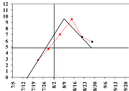
Figure 2. COTMAN growth curve for late-planted cotton. Halfway, TX.
