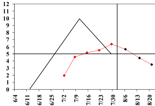
Figure 6. COTMAN growth curve under a 30-inch row spacing. Halfway, TX.
