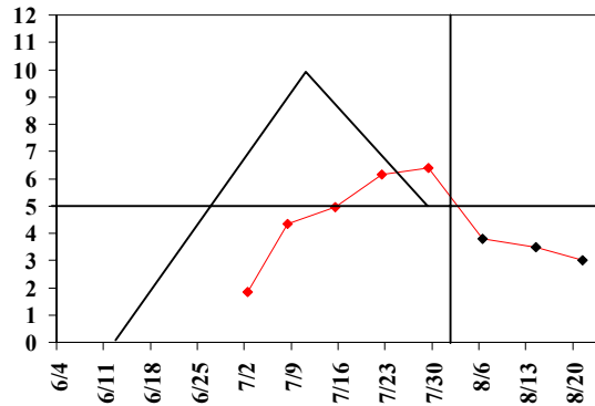
Figure 5. COTMAN growth curve under a 15-inch row spacing. Halfway, TX.
