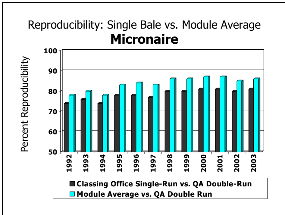
Figure 1. Reproducibility of Micronaire 1992-2003.
