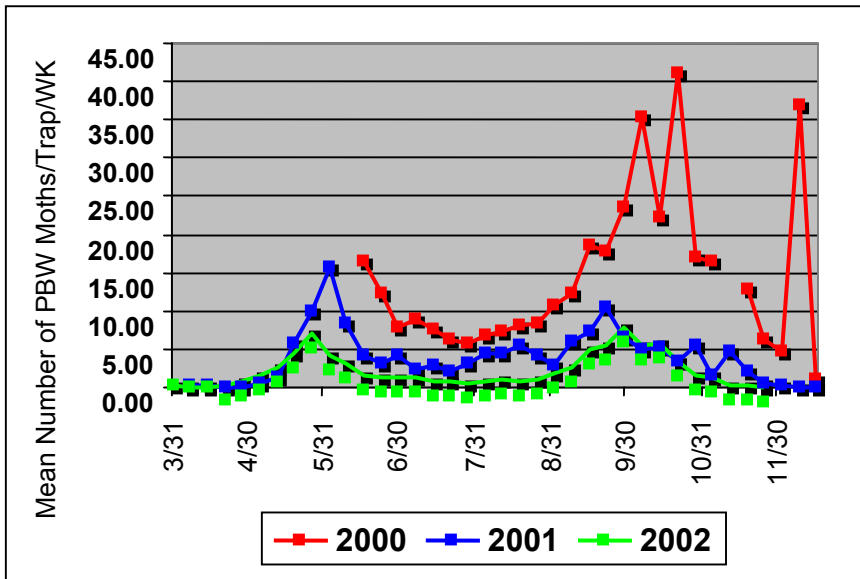
Figure 2. Weekly PBW Trapping, El Paso/Trans Pecos, Texas, 2000, 2001, and 2002.
