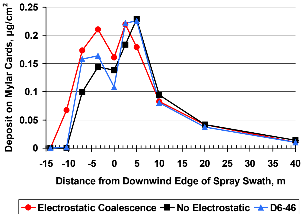
Figure 3. Displaced swath and near-field spray deposits.
