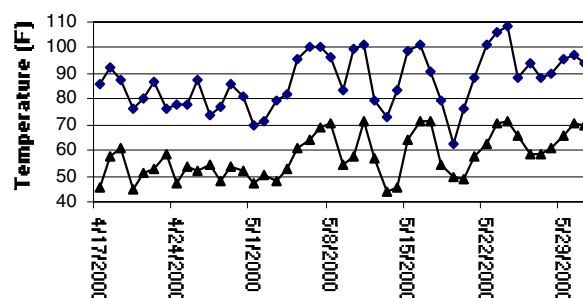
Figure 1. Minimum and maximum air temperature for spring 2000.
