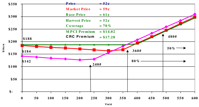
Figure 5. Payoff Function: Catastrophic, Multi-Peril, and Crop Revenue Coverage.
