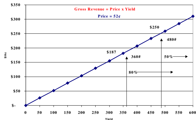
Figure 1. Payoff Function: No Insurance.
