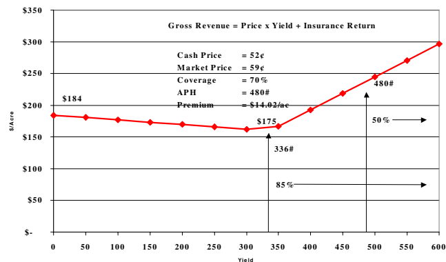
Figure 3. Payoff Function: Multi-Peril Crop Insurance.
