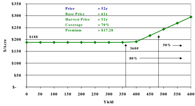
Figure 4. Payoff Function: Crop Revenue Coverage.
