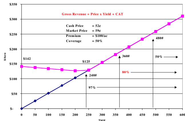
Figure 2. Payoff Function: Self Insurance Versus Catastrophic.
