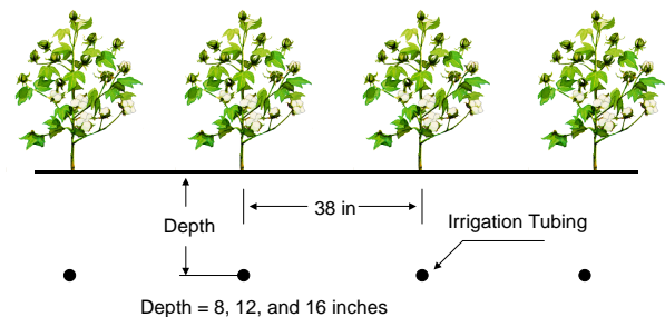
Figure 1. Drip irrigation lateral spacing and depth configuration (subsurface every row).
