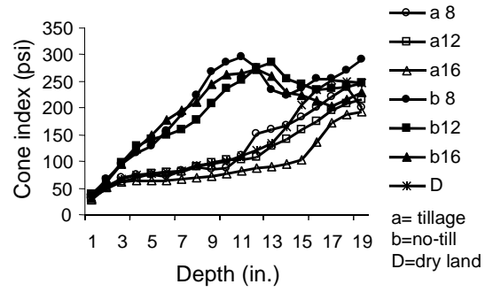
Figure 3. Effects of tillage and irrigation on soil compaction.
