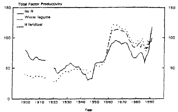
Fig. 6. Total factor productivity indexes for the 3 continuous cotton treatments (cotton planted every year) relative to 1990's index. The large increase in relative TFP around 1960 was due to the introduction of the mechanical cotton picker (from Traxler et al., 1995).
