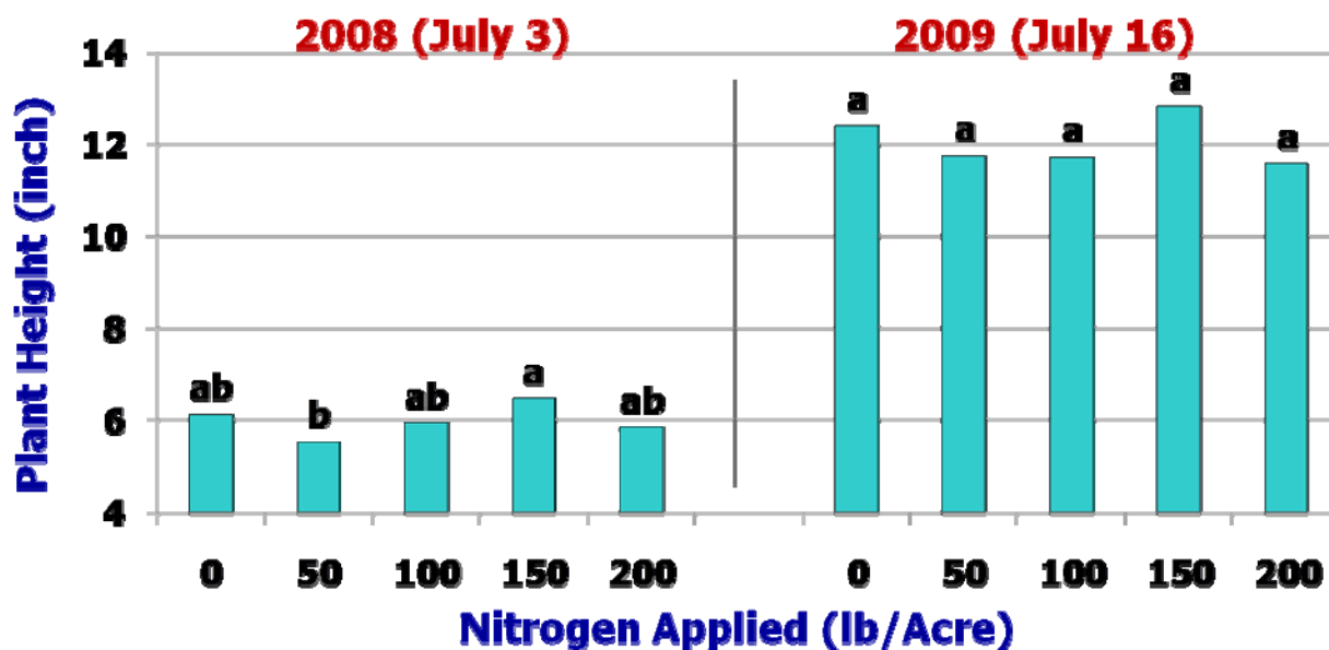
Figure 2. Effect of residual soil nitrogen on early plant growth as measured by plant height, 2008-2009.
