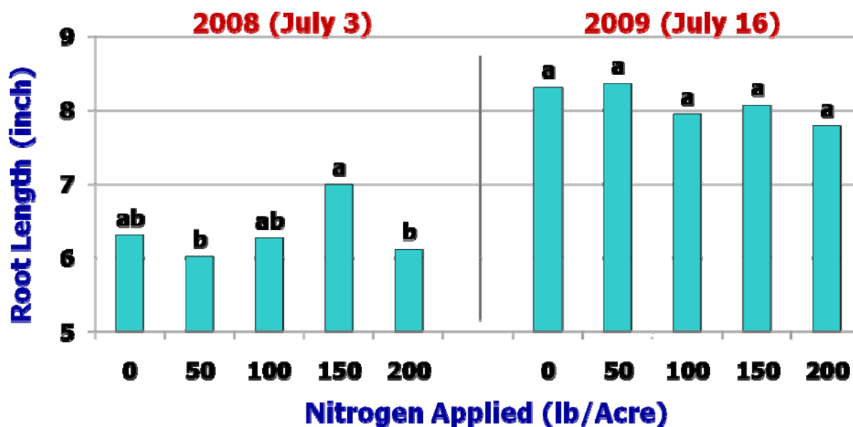
Figure 3. Effect of residual soil nitrogen on early plant growth as measured by root length, 2008-2009.
