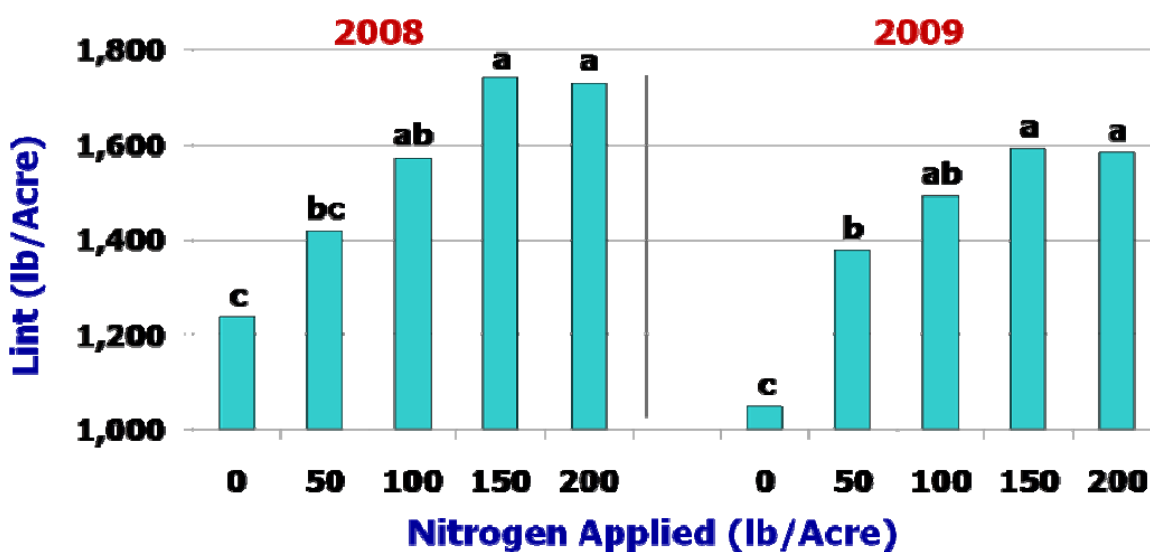
Figure 7. Effect of variable rates of soil applied nitrogen on cotton lint yield, 2008-2009.
