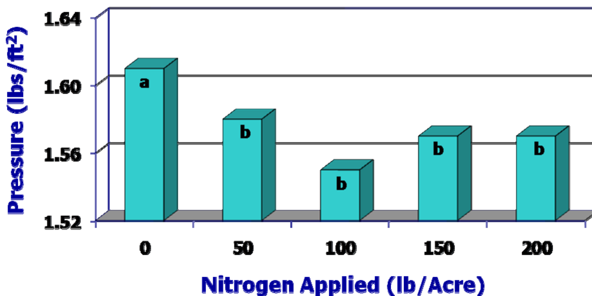
Figure 6. Amount of pressure required to puncture the carpal wall of cotton bolls aged to 350 heat units (>60 °F) as affected by variable nitrogen rates applied to the soil in replicated experimental plots, 2009.
