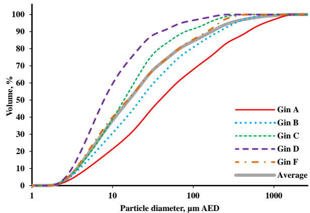
Figure 5. Gin average cumulative particle size distributions for the PM captured on a EPA-Method 17 filter from the 2 nd stage mote systems.
