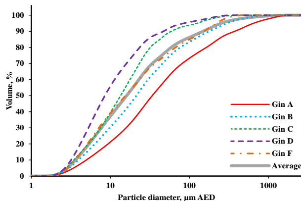
Figure 7. Gin average cumulative particle size distributions for the EPA-Method 17 combined filter and wash samples from the 2 nd stage mote systems.
