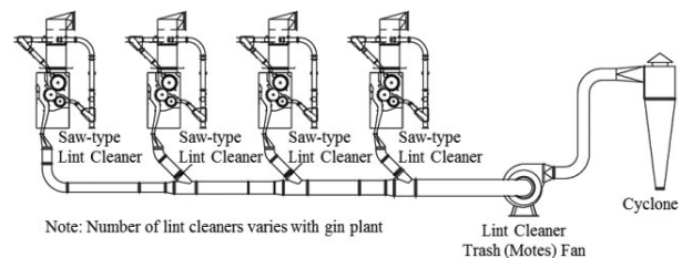
Figure 2. Typical cotton gin 2 nd stage mote system layout (Courtesy Lummus Corporation, Savannah, GA).
