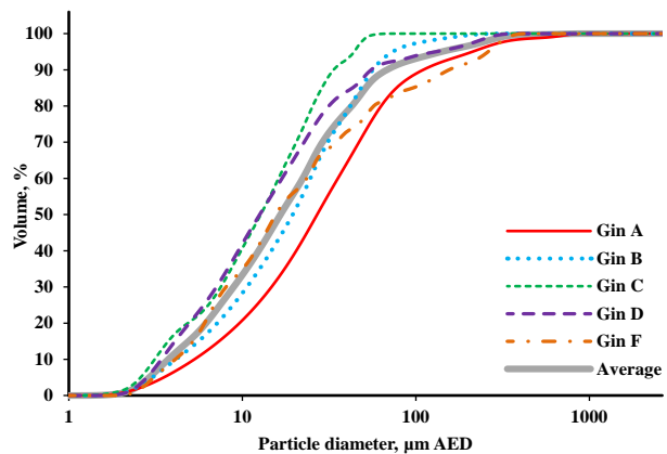
Figure 6. Gin average cumulative particle size distributions for the PM captured in the EPA-Method 17 sampler nozzle wash from the 2 nd stage mote systems.
