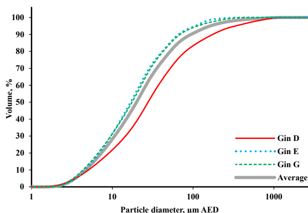
Figure 7. Gin average cumulative particle size distributions for the EPA-Method 17 combined filter and wash samples from the combined lint cleaning systems.
