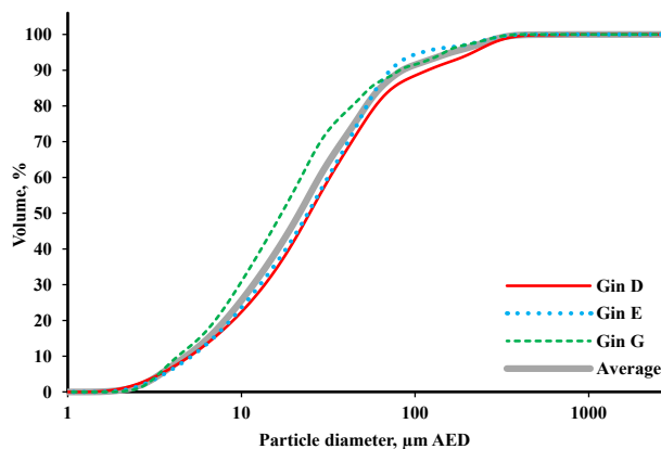
Figure 6. Gin average cumulative particle size distributions for the PM captured in the EPA-Method 17 sampler nozzle wash from the combined lint cleaning systems.
