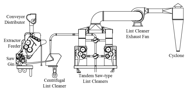
Figure 2. Typical cotton gin combined lint cleaning system layout (Courtesy Lummus Corporation, Savannah, GA).
