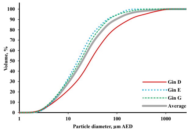
Figure 5. Gin average cumulative particle size distributions for the PM captured on a EPA-Method 17 filter from the combined lint cleaning systems.
