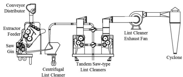
Figure 2. Typical cotton gin 2 nd stage lint cleaning system layout (Courtesy Lummus Corporation, Savannah, GA).
