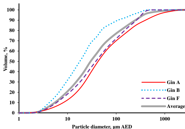
Figure 7. Gin average cumulative particle size distributions for the EPA-Method 17 combined filter and wash samples from the 2 nd stage lint cleaning systems.
