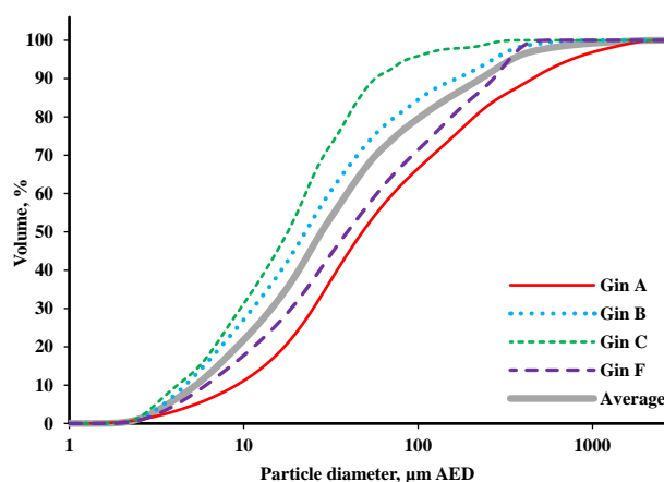
Figure 5. Gin average cumulative particle size distributions for the PM captured on a EPA-Method 17 filter from the 2 nd stage lint cleaning systems.
