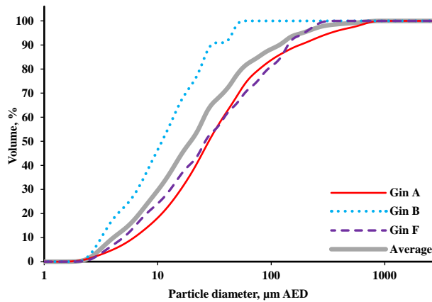
Figure 6. Gin average cumulative particle size distributions for the PM captured in the EPA-Method 17 sampler nozzle wash from the 2 nd stage lint cleaning systems.
