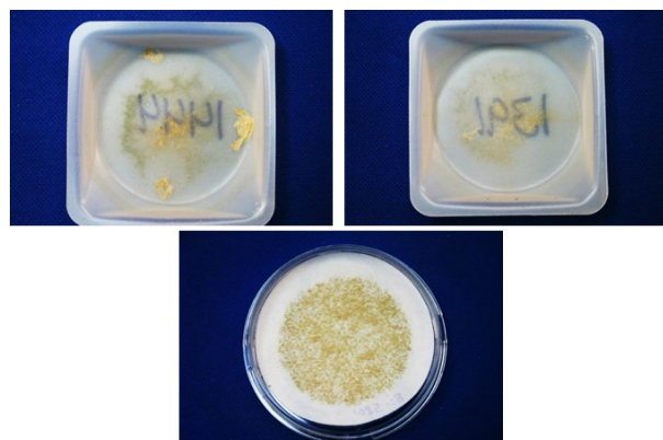
Figure 13. Typical EPA Method 201A filter and sampler head acetone washes from the 1 st stage lint cleaning system. Clockwise from top left: > 10 µm wash, ≤ 10 µm wash, and filter.
