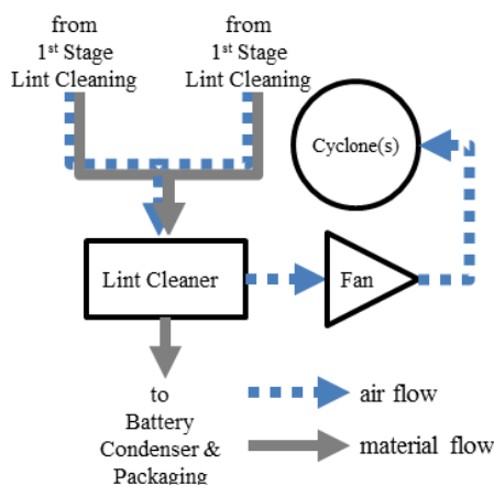
Figure 11. Schematic of 2 nd stage lint cleaning system preceded by double 1 st stage lint cleaning systems (gin B).
