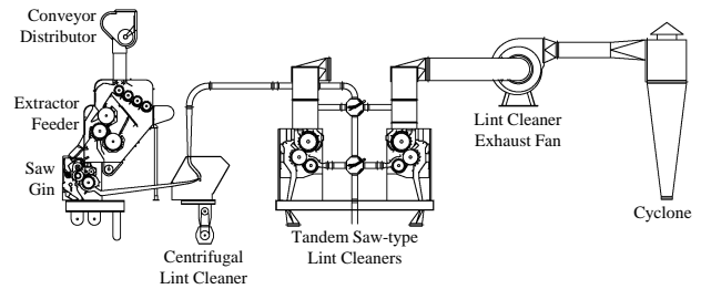
Figure 3. Typical cotton gin 2 nd stage lint cleaning system layout (Courtesy Lummus Corp., Savannah, GA).
