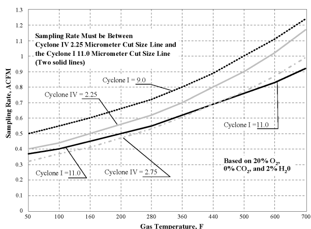
Figure 7. Acceptable sampling rate for combined cyclone heads (CFR, 2010). Cyclone I = PM 10 sizing cyclone and Cyclone IV = PM 2.5 sizing cyclone (gas temperatures for the 2 nd stage lint cleaning systems tested ranged from 19 to 42°C [67-107°F]).
