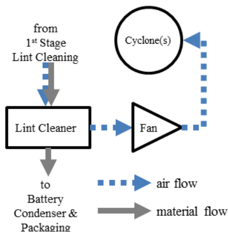
Figure 10. Schematic of 2 nd stage lint cleaning system preceded by single 1 st stage lint cleaning system (gins A, C, and F).
